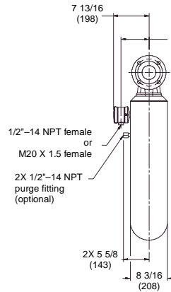
CMF300 with junction box
