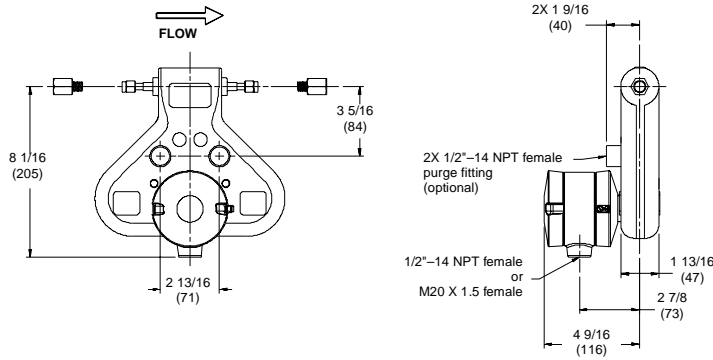
CMF010 with junction box
