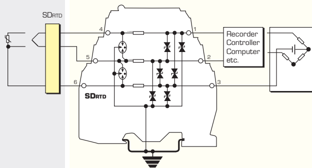
3 wire RTDs
