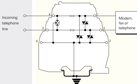
Telecom line
