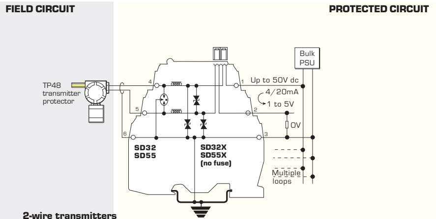
2-wire transmitters
