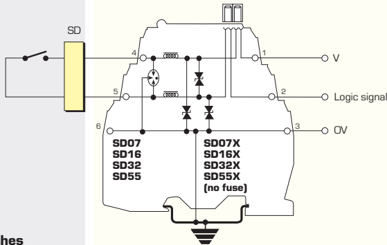
Switches
